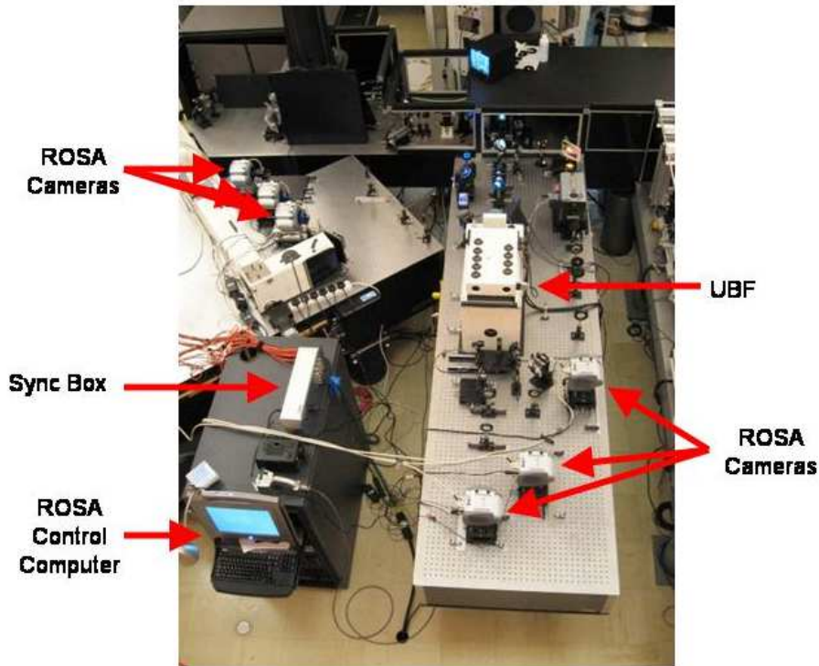
Figure 1. Six ROSA cameras placed on two optical benches at the DST during the commissioning run in August 2008. Three cameras are positioned behind “blue” filters (G-band, 4170 Å continuum and Ca-K core; left optical bench), while the remaining three cameras are positioned behind “red” filters (H \alpha core and circularly polarized measurements at 6302 Å; right optical bench). One of the rack-mounted storage assemblies is also visible towards the lower-left side of the image.
