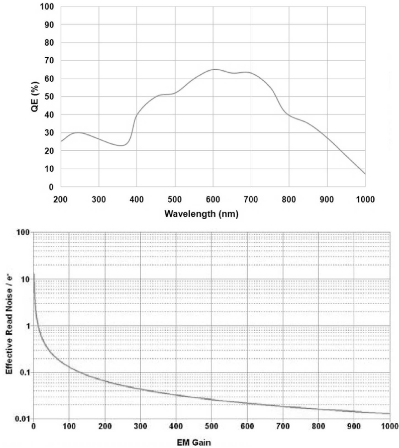
Figure 2. Upper panel is a representation of a ROSA camera’s quantum efficiency as a function of wavelength, while the bottom panel plots a ROSA camera’s effective read noise as a function of electron-multiplying gain. In this instance, the effective read noise is a combination of CCD readout noise and analogue-to-digital convertor noise.
